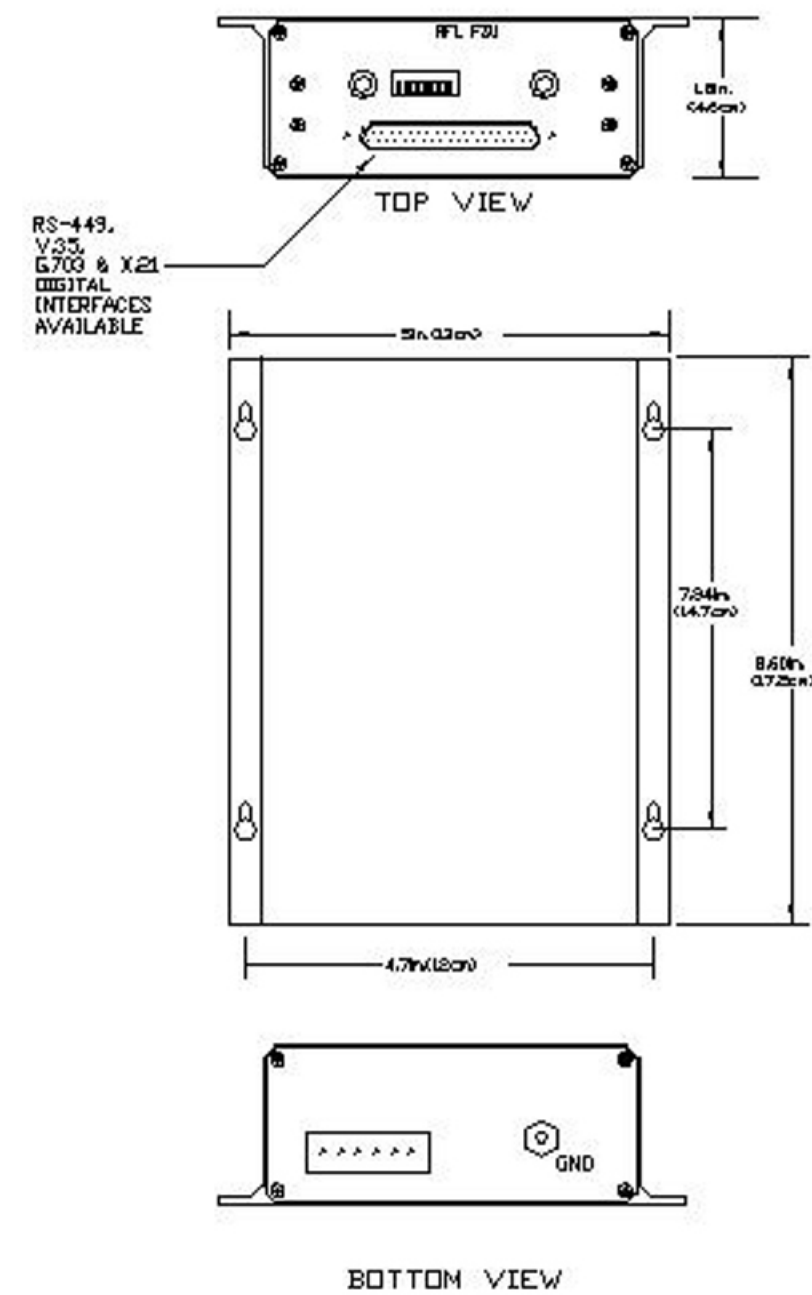
REMOTE FIBER OPTIC SERVICE UNIT
