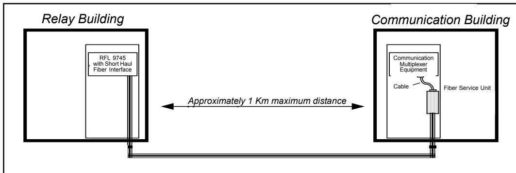
Figure 4. Typical RFL 9745 Short Haul Fiber Optic Application with Fiber Service Unit
