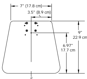
Base Plate (Reduced scale)
