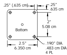
Universal Stand Base
