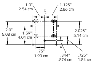
Base Plate Hole Pattern
