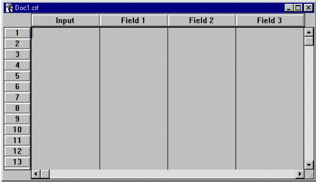
Figure 2-70 CRF Window
