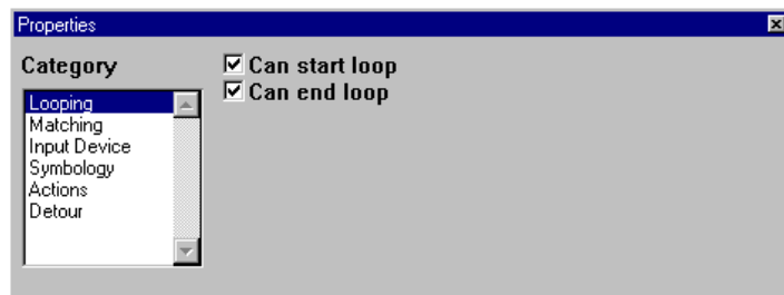
Figure 2-16 Looping Property
