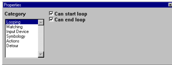
Figure 2-15 Properties Window
