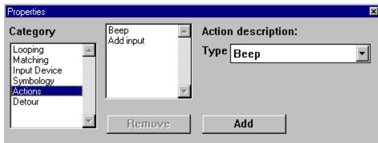
Figure 2-36 Actions Property
