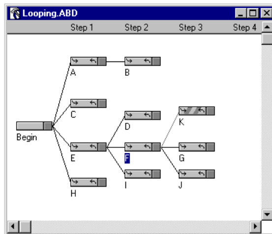
Figure 2-18 Loop Example
