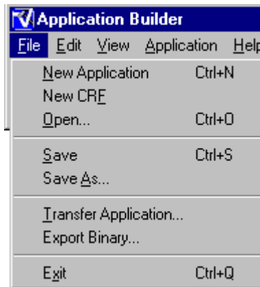
Figure 2-2 File Menu
