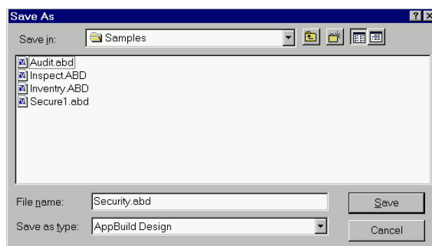
Figure 3-6 Name Application
