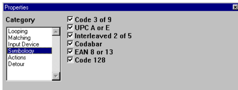
Figure 2-34 Symbology Property
