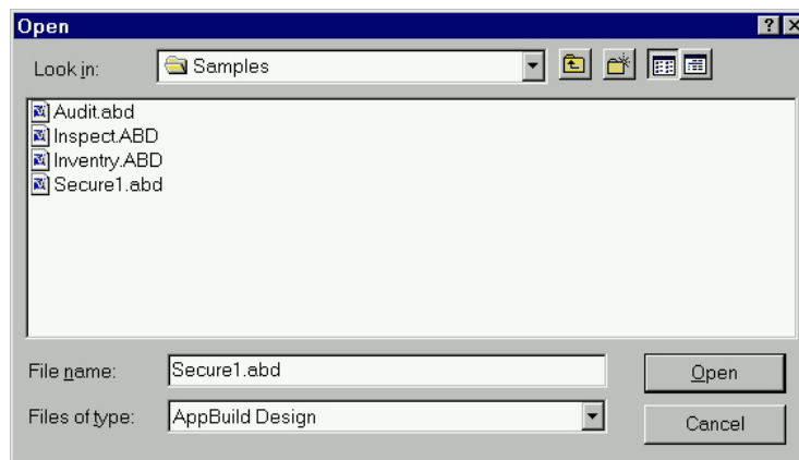
Figure 1-7 Open Secure1.abd
