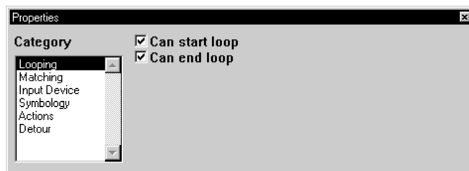
Figure 4-42 Properties Window
