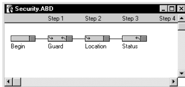
Figure 4-1 Security.abd Application
