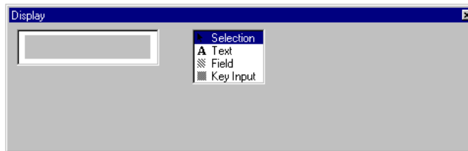
Figure 3-59 Display Window
