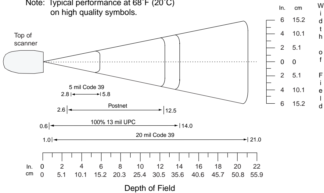
Figure 2-7 Symbol DS6608 Standard Range Digital Scanner Decode Zone for 1D Bar Codes
