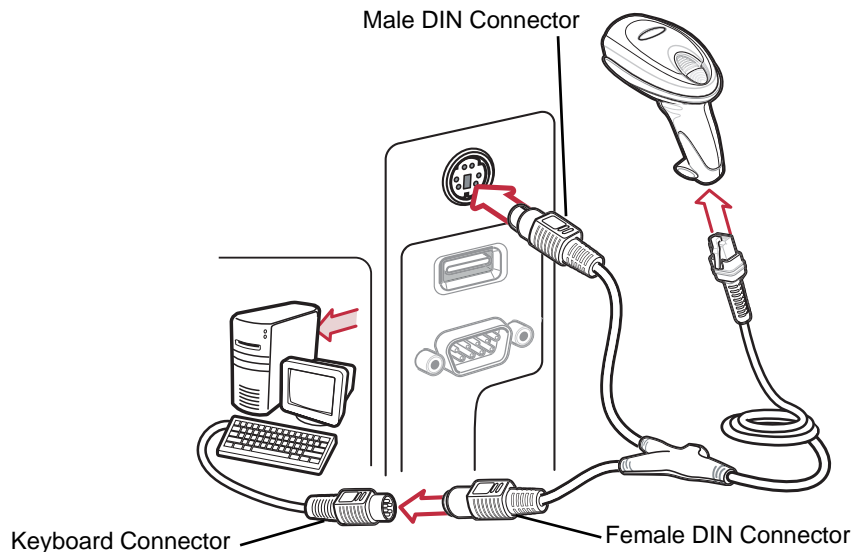
Figure 6-1 Keyboard Wedge Connection with Y-cable
