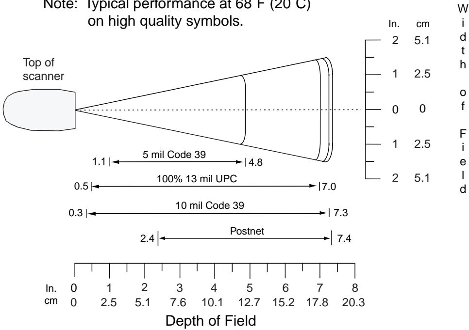
Figure 2-9 Symbol DS6608 High Density Digital Scanner Decode Zone for 1D Bar Codes
