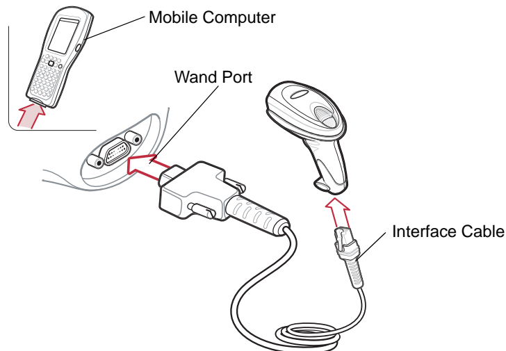
Figure 10-1 Wand Emulation Connection
