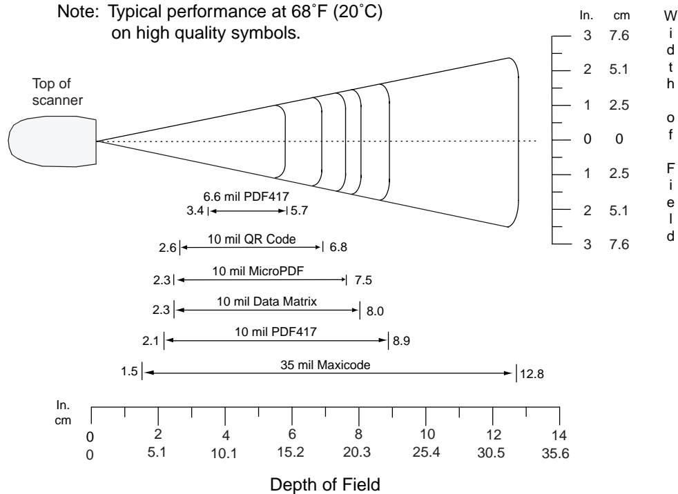
Figure 2-8 Symbol DS6608 Standard Range Digital Scanner Decode Zone for 2D Bar Codes
