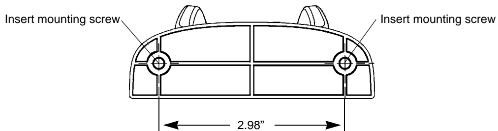
Figure 1-7 Wall Mounting Template
