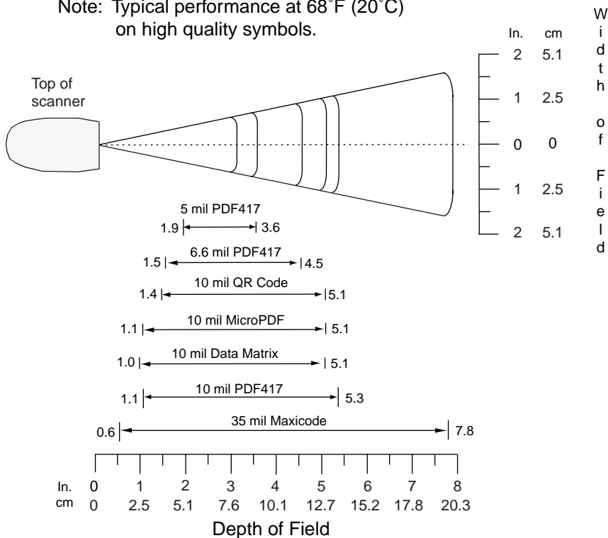
Figure 2-10 Symbol DS6608 High Density Digital Scanner Decode Zone for 2D Bar Codes
