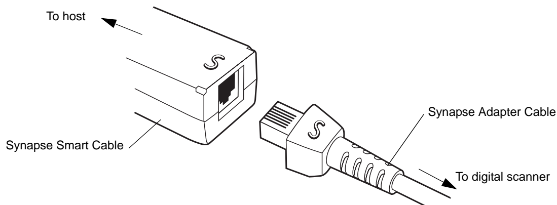
Figure 1-4 Synapse Cable Connection
