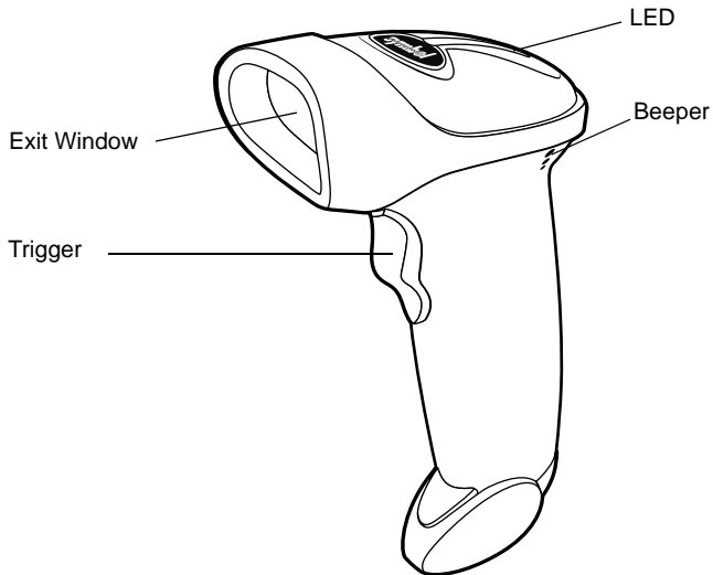
Figure 2-1. Scanner Parts
