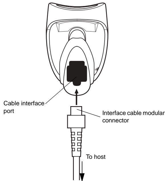
Figure 1-2. Installing the Cable
