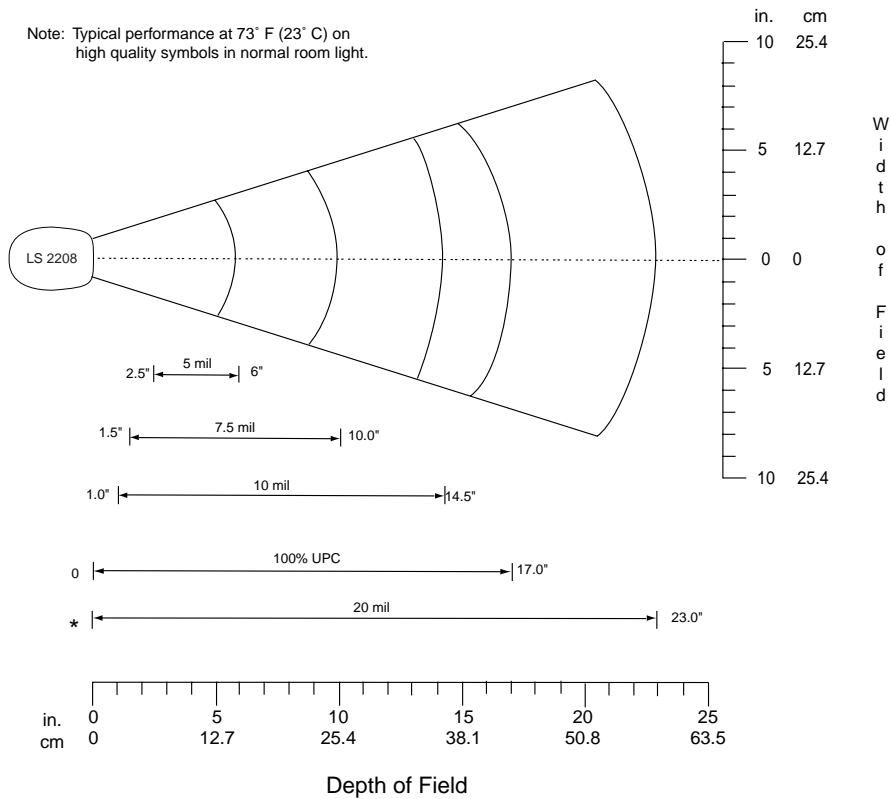
Figure 2-4. LS 2200/2208 Decode Zone
