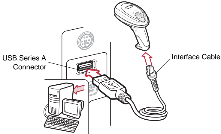
Figure 7-1 USB Connection
