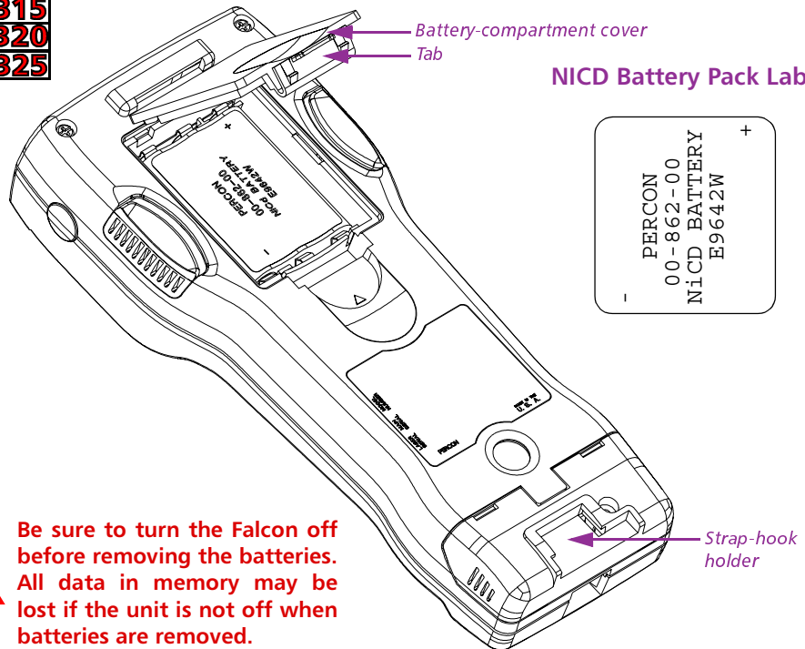
Figure 2-1: NiCD Battery Pack in Falcon 310 , 315 , 320 , or 325 Battery Compartment
