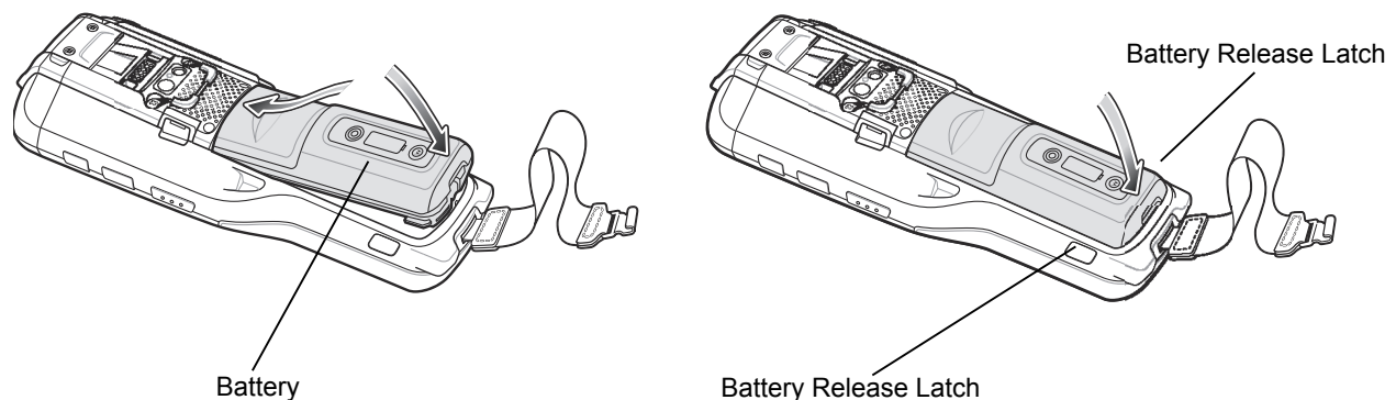
Figure 1-11 Inserting the Battery
