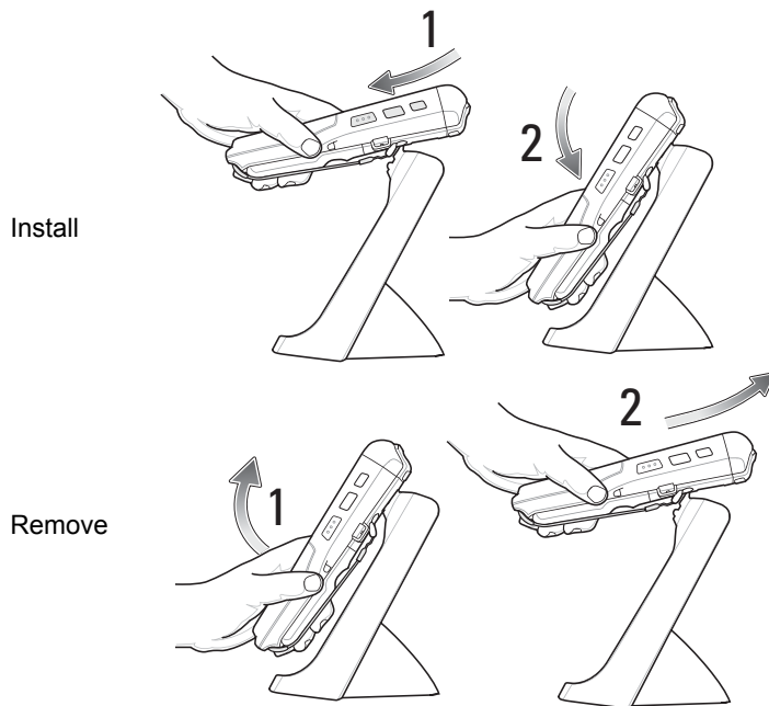
Figure 8-1 Hooking the MC9500-K onto the Single Bay USB Cradle
