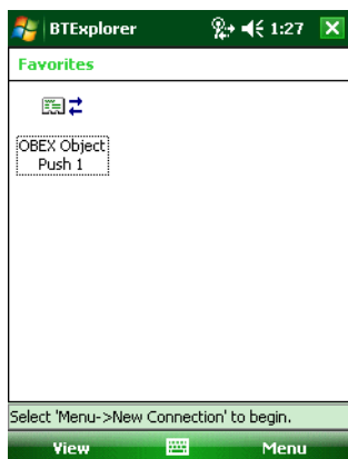
Figure 7-22 Favorites Window
