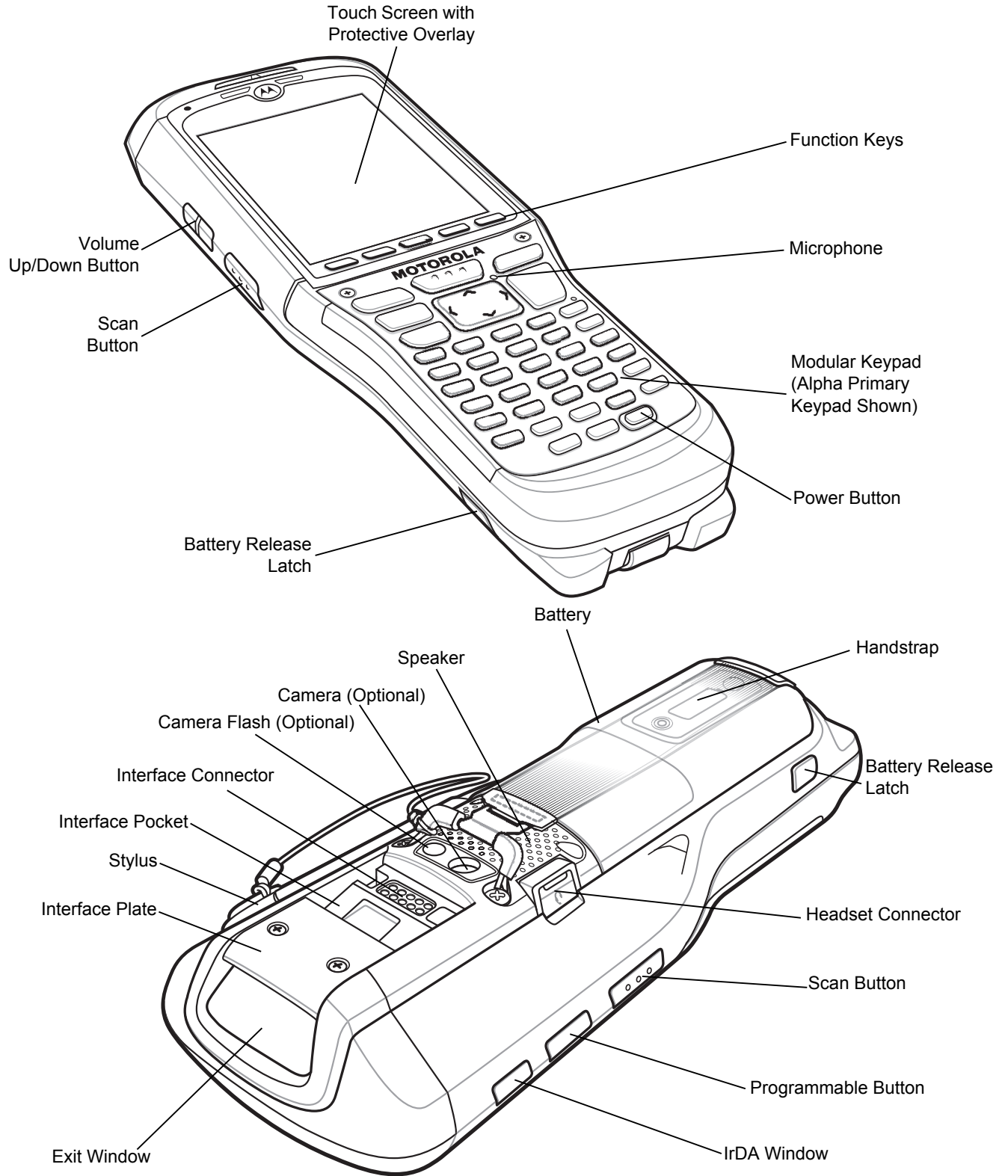
Figure 1-1 MC9500-K
