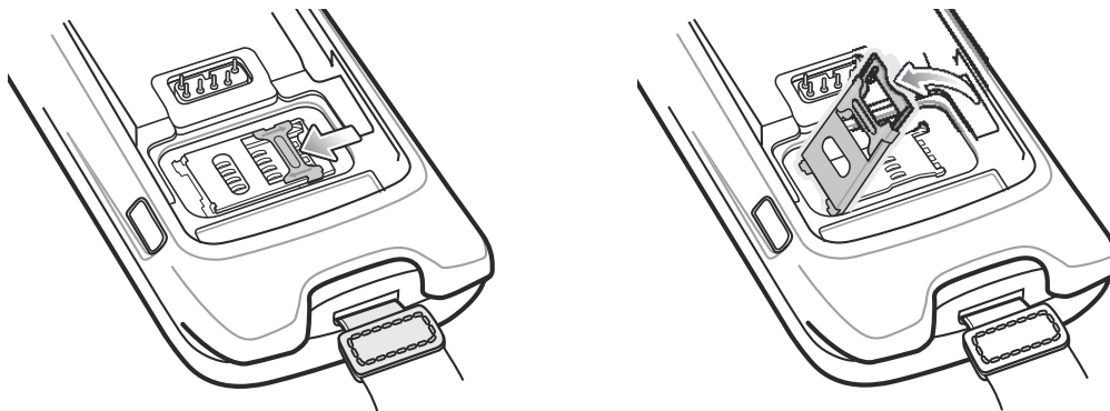
Figure 1-9 Lifting the SIM Cover
