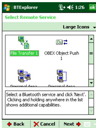
Figure 7-20 Device Services
