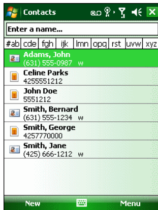
Figure 5-18 Contacts
