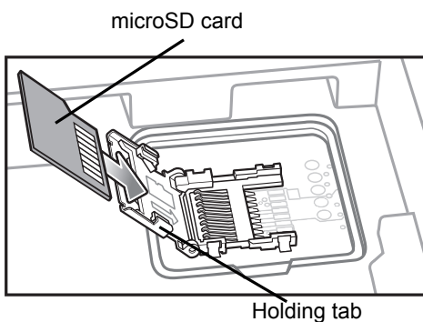
Figure 1-4 Insert microSD Card in Holder
