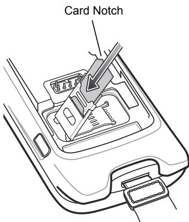
Figure 1-10 Inserting the SIM Card
