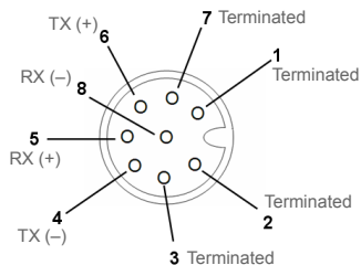
Connector B (Ethernet Models) M12 8-pin Socket
