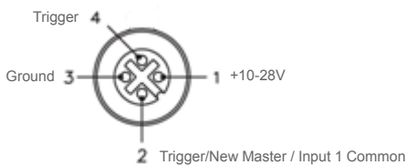
Connector T (Trigger) 4-pin Socket
