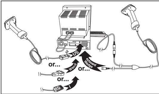
Figure 2. Other Interface Connections
